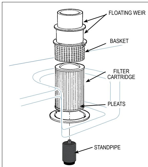
FILTER SYSTEM
