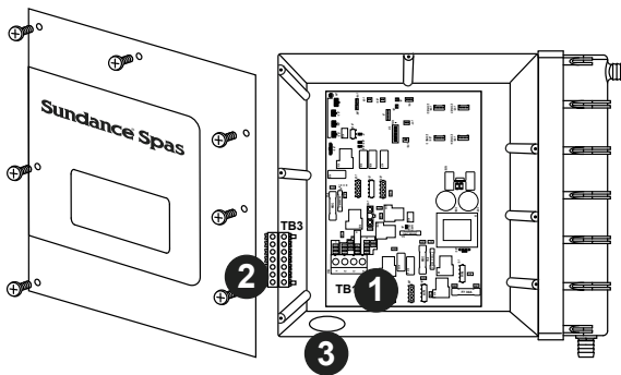
Figure C Control Box
